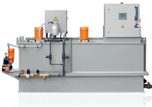
Metering system Ultromat® ULFa (continuous flow system)
