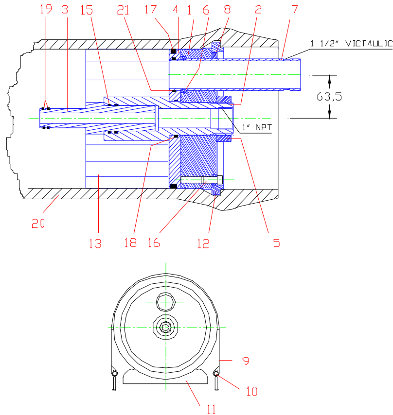
ASSEMBLY DRAWING OI8040nb : 800001
