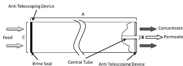
Figure 1: Element Dimensions Diagram, Female 8040
