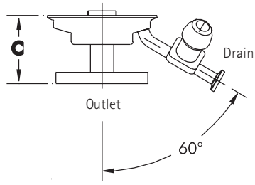
In-line Base with Flange Outlet Connection
