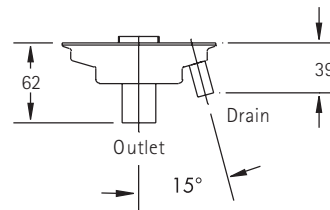
In-line Base with Butt Weld Outlet Connection
