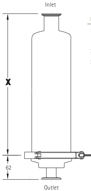
In-line Housing with Ferrule Outlet Connection
