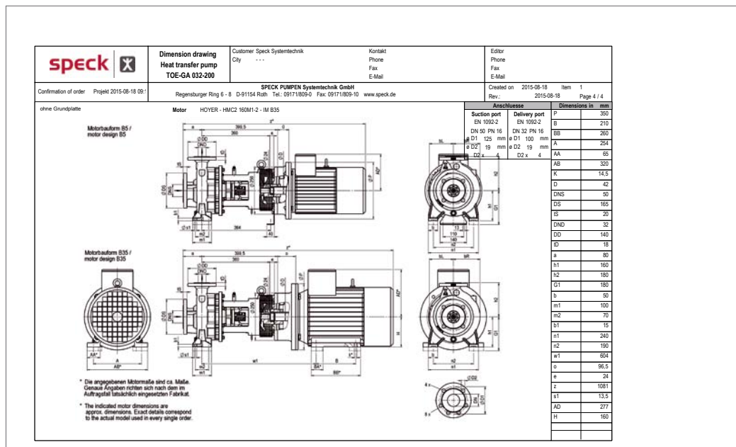
Dimensional drawing (example)
