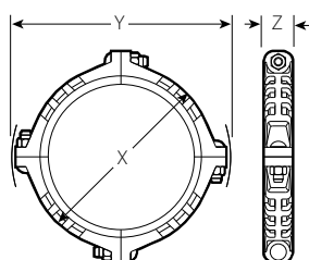
16 – 18"/400 – 450 mm SIZES
