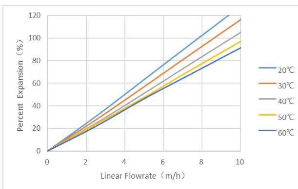
Fig. 2 Backwash Expansion
