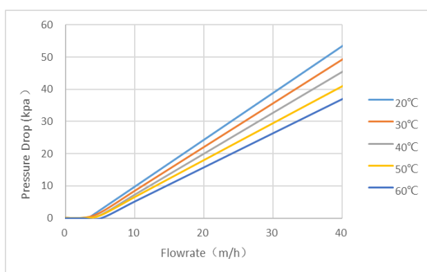
Fig. 1 Pressure Drop
