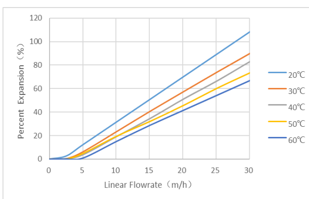
Fig. 2 Backwash Expansion
