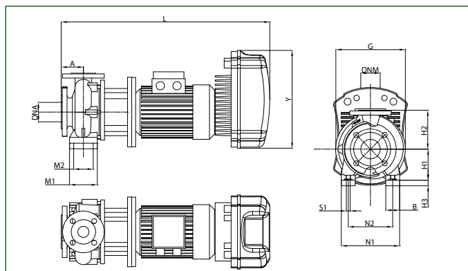
NKP-GE 40-125/130
