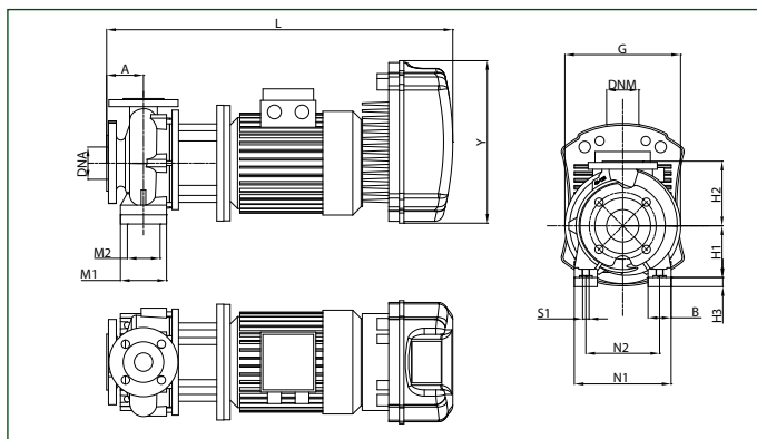
NKP-GE 40-125/139 - NKP-GE 40-160/158
