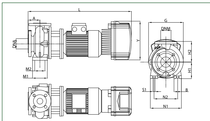
NKP-GE 40-125/120
