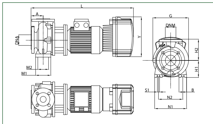
NKP-GE 40-125/107
