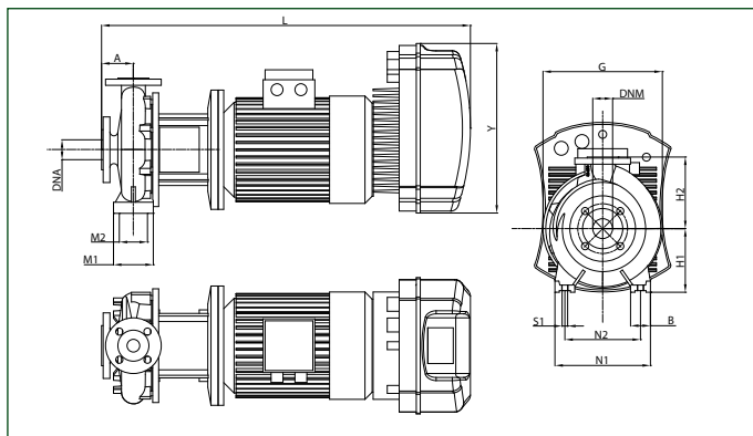
NKP-GE 32-200/210
