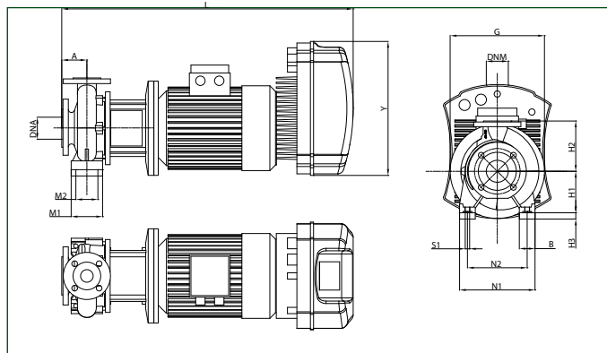
NKP-GE 40-160/172 - NKP-GE 40-200/210
