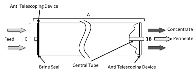
Figure 1b: Element Dimensions Diagram – Male
