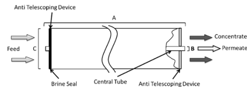
Figure 1b: Element Dimensions Diagram – Female
