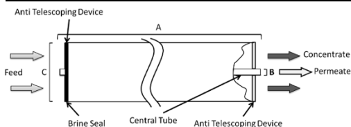
Figure 1: Element Dimensions Diagram – Male
