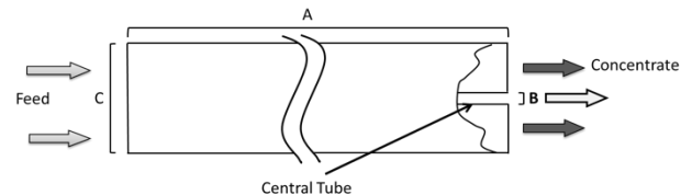
Figure 2: Element Dimensions Diagram – All Except 8040
