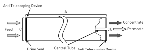
Figure 2: Element Dimensions Diagram (Female) – 8040
