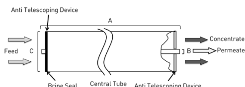
Figure 1: Element Dimensions Diagram (Male) – 2540 &amp; 4040
