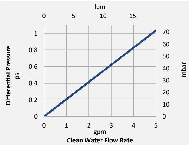
Graph 1: Muni.Z clean water flow rate based on a 10 in length filter
