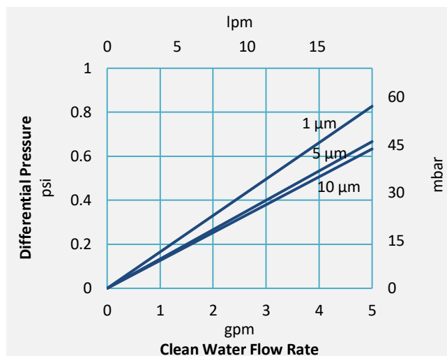
Graph 1: Purtex Plus clean water flow rate based on a 10 in length filter
