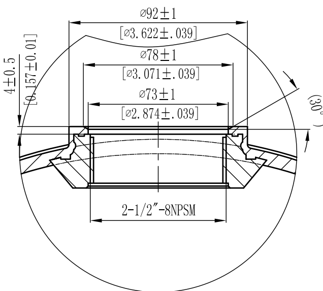
A DETAIL 1:2
