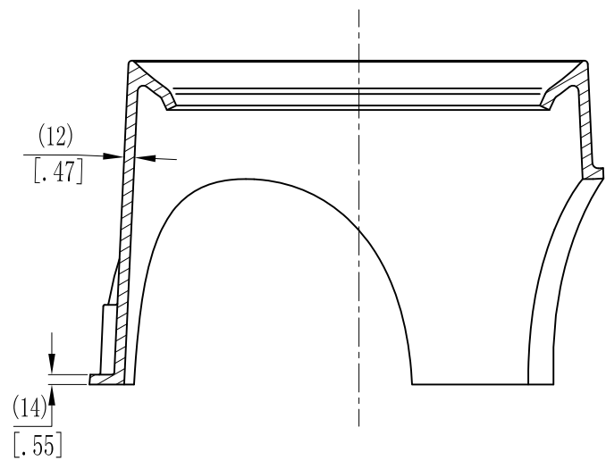
B-B ROTATING VIEW
