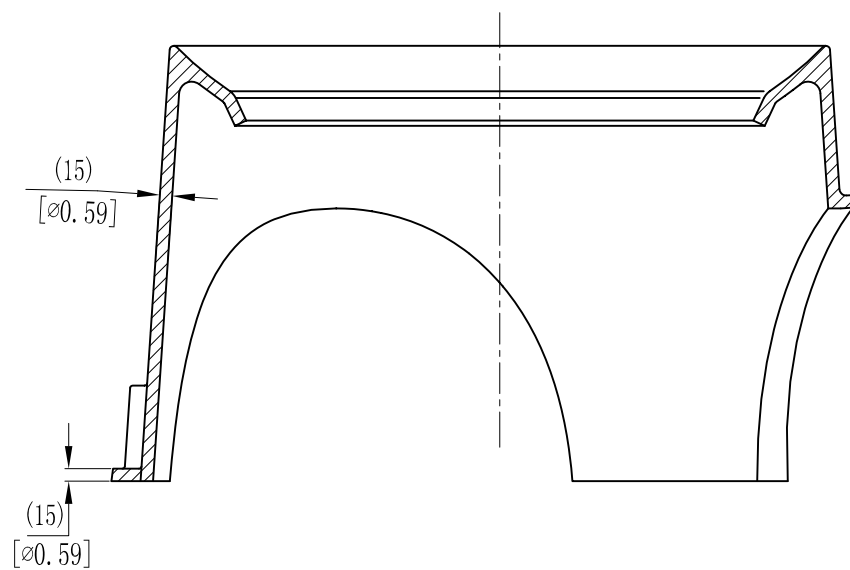
B-B ROTATING VIEW
